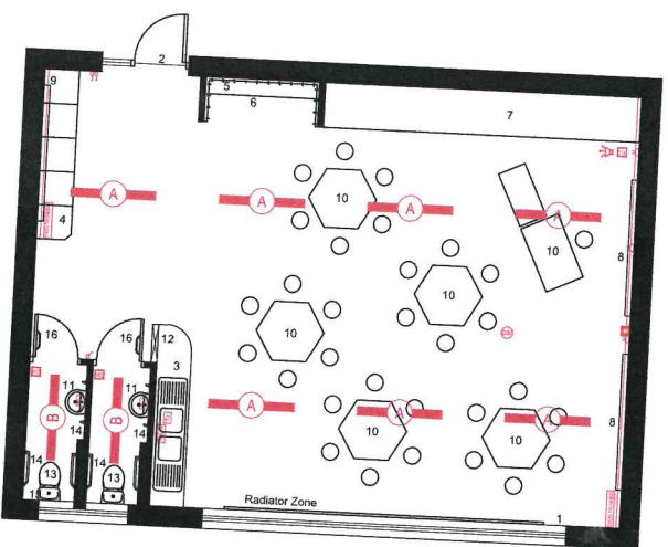
PROPOSED CLASSROOMS TYPICAL FLOOR PLANS (209SQM)
